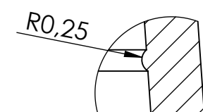
DETAIL E SCALE 10 : 1
